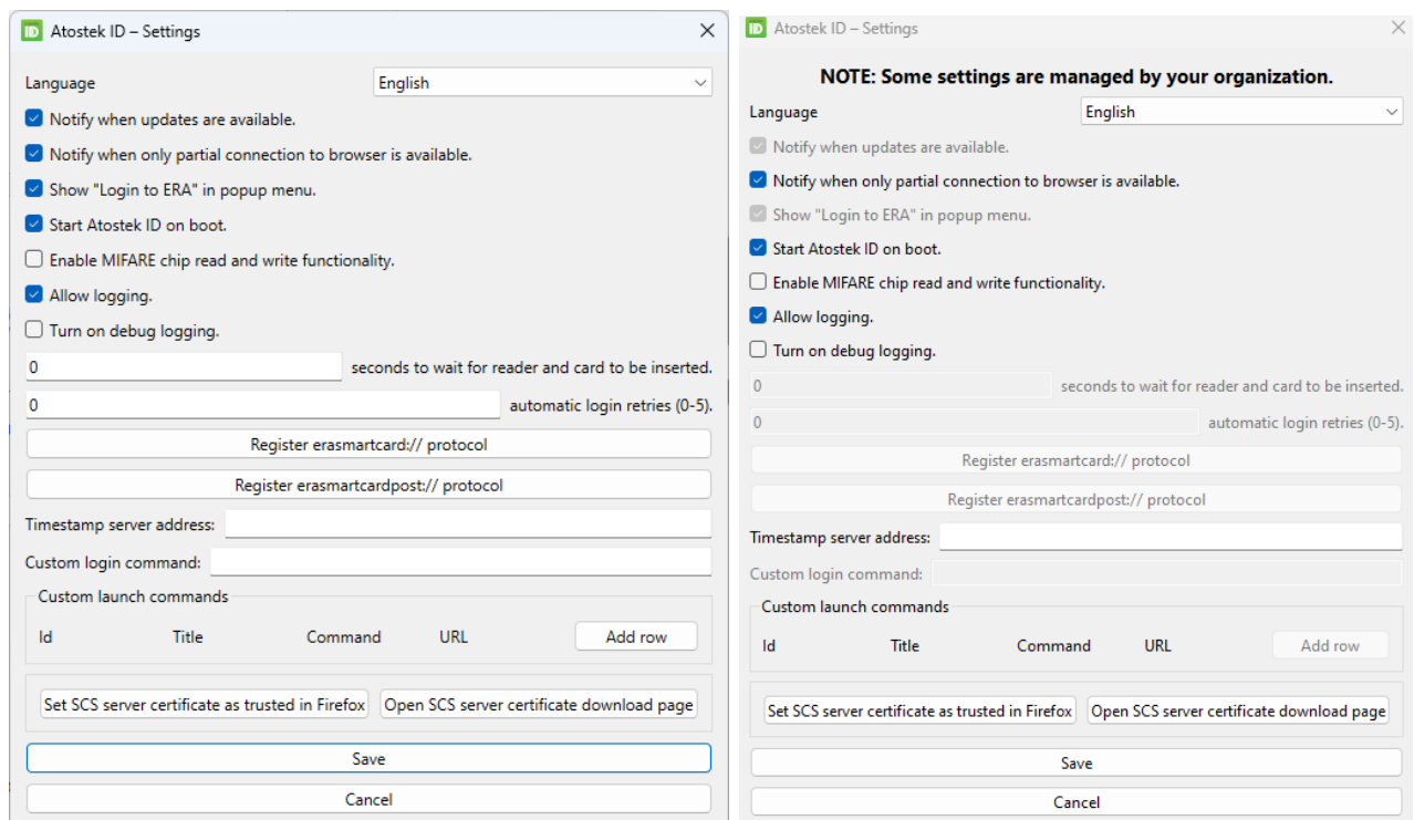
Figure 8: On the left is the default view of the settings, and on the right is the settings dialog when the organization manages some of the application's settings on behalf of the user.
